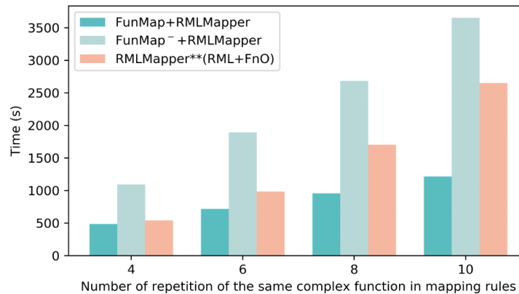
(c) RMLMapper - 25% of duplicates
