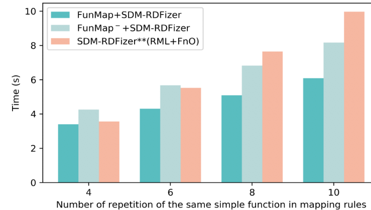
(b) SDM-RDFizer - 75% of duplicates
