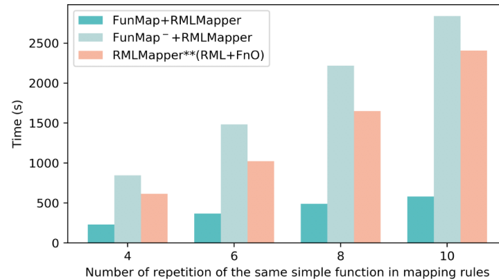
(c) RMLMapper - 25% of duplicates
