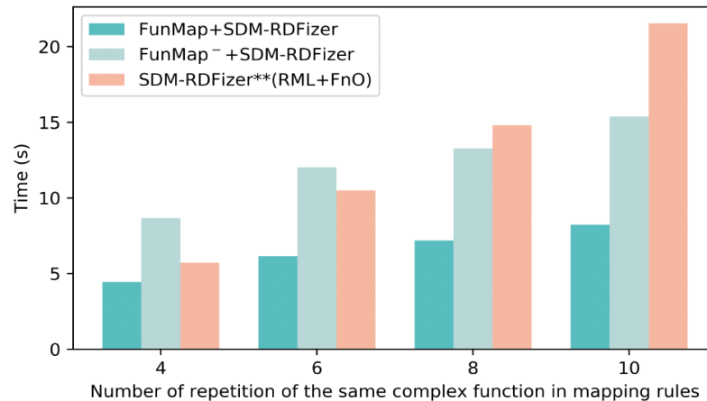
(a) SDM-RDFizer - 25% of duplicates
