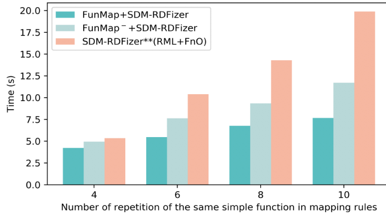
(a) SDM-RDFizer - 25% of duplicates
